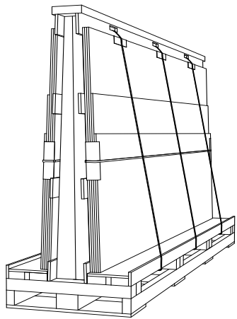
Wooden A-frame
